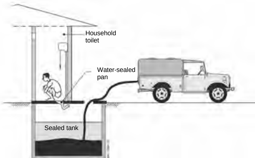
Figure 22.2. Vault latrine
