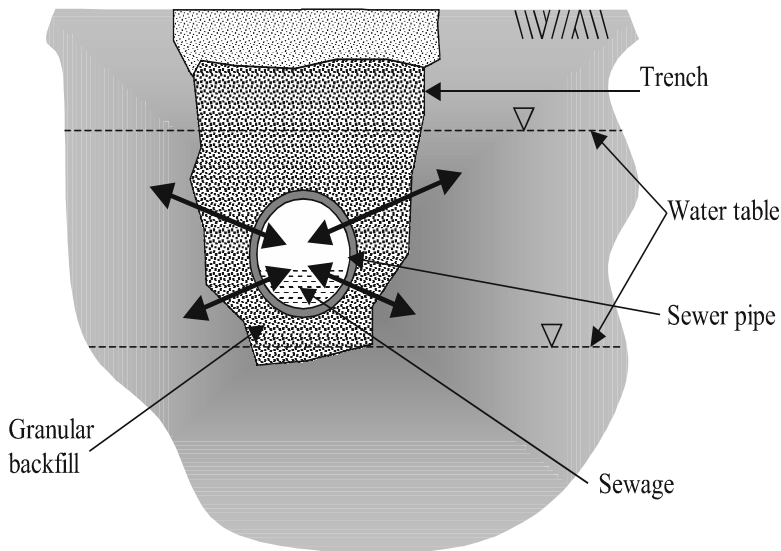
Figure 10.2. Sewer design
